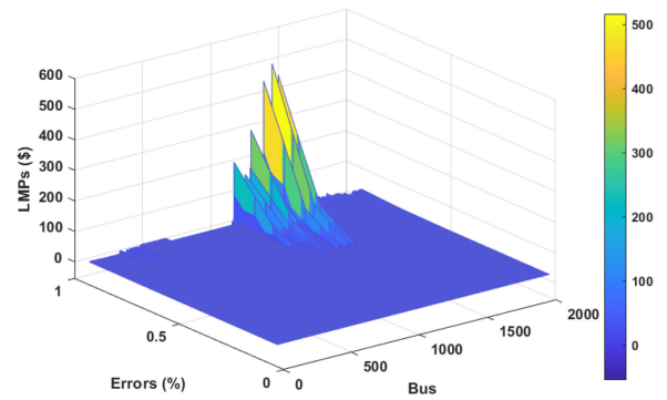
Fig. 7. LMP incremental due to low-quality renewables.
