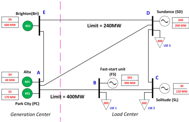
Fig. 2. PJM-5 bus system with 70% renewable penetration.
