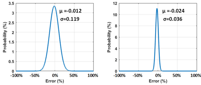
Fig. 6. Deviation distribution for renewables and LSEs.
