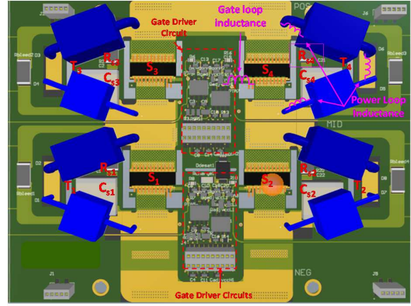
Fig. 9. Layout of the proposed SSCB
