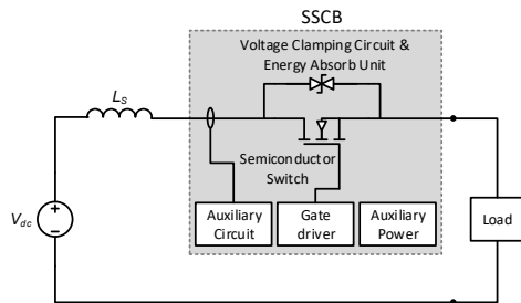
Fig. 1. Typical SSCB in a DC system
