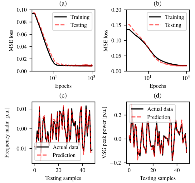
Fig. 5. DNN training results: (a) Training loss of frequency nadir prediction; (b) Training loss of IBR peak power prediction; (c) Testing of frequency nadir prediction; (d) Testing of IBR peak power prediction.
