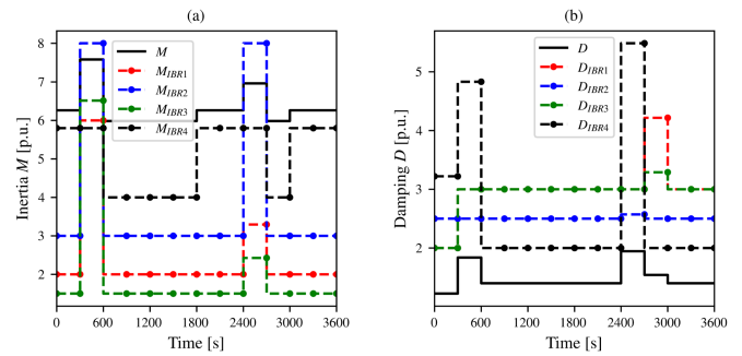
Fig. 11. IBRs inertia and damping: (a) virtual inertia; (b) virtual damping.
