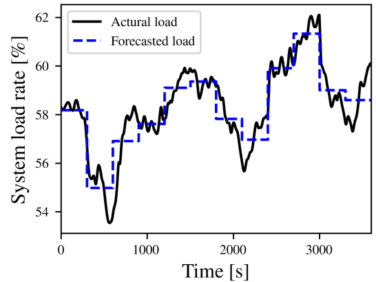
Fig. 8. One-hour load profile.
