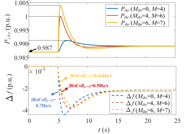
Fig. 6. Dynamic performance of the two-machine system with VIS-RTED scheduling results.
