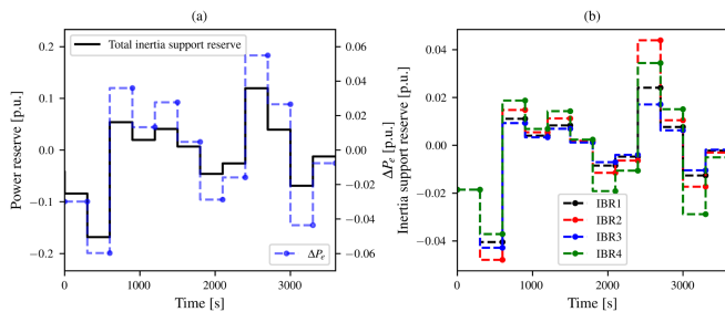
Fig. 10. IBRs inertia support reserve: (a) total reserve along with \Delta P_e ; (b) single IBR reserve.
