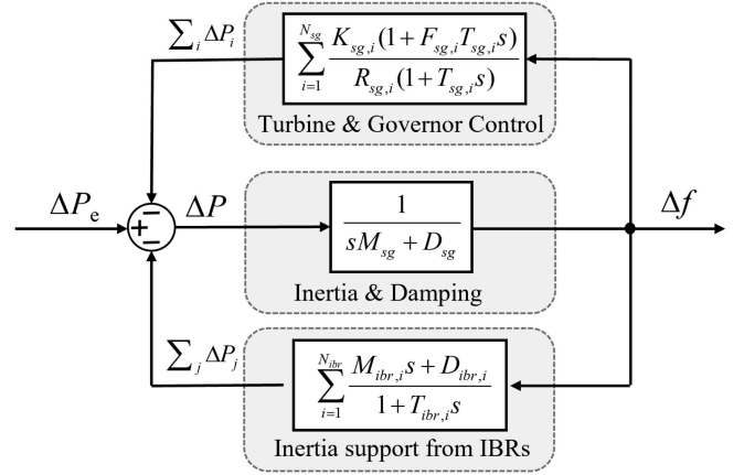
Fig. 2. Uniform frequency dynamics model of IBR-penetrated power system [15].
